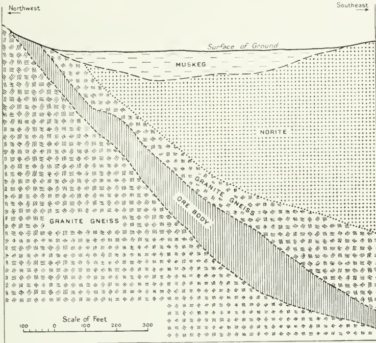
Fig. 40—Levaek ore body, Sudbury area, Ontario, showing how the deposit occurs in the granite-gneiss.
